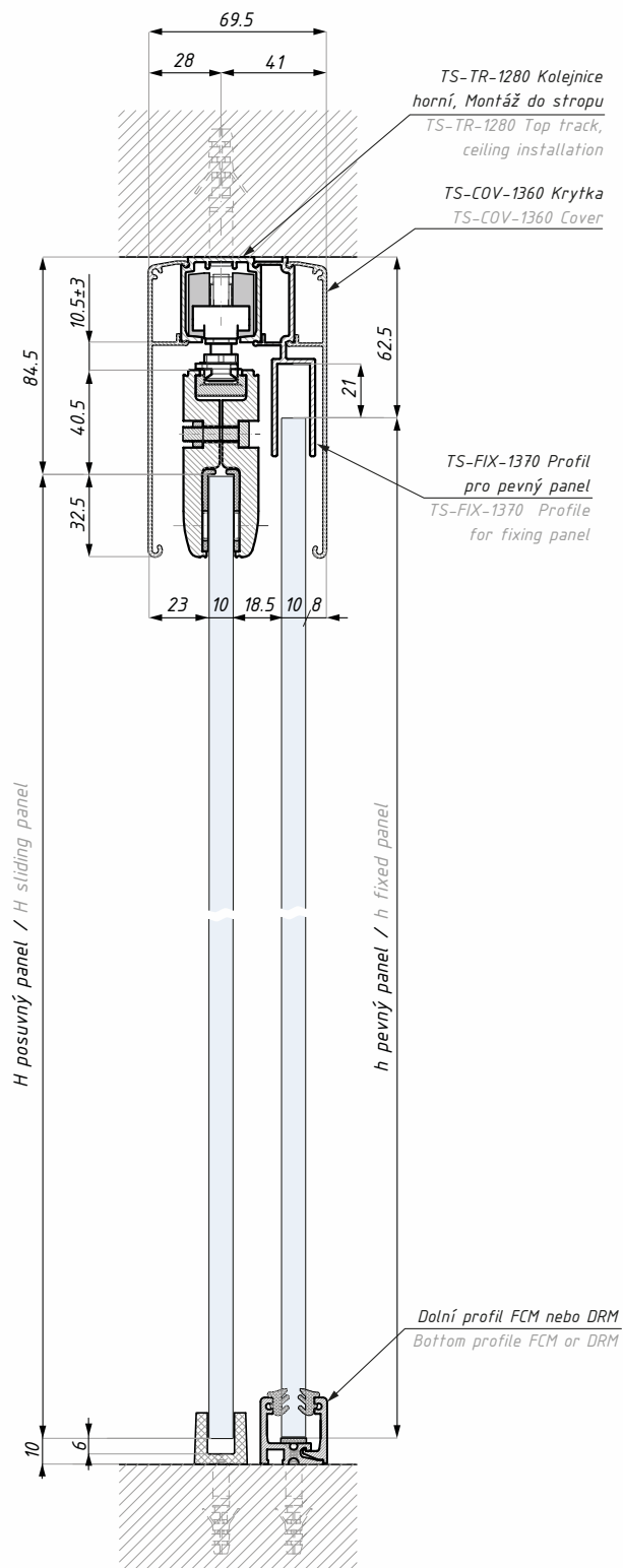
Montáž do stropu s pevným panelem Installation to the ceiling with fixed panel
