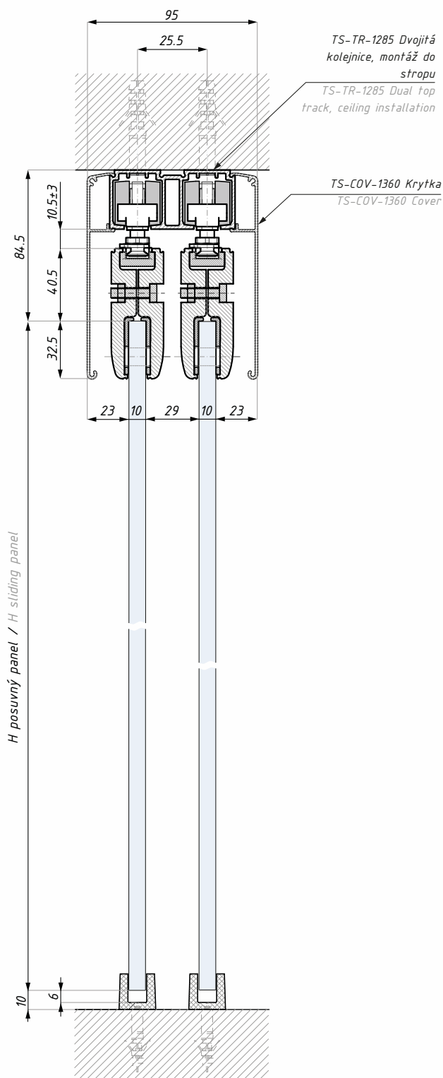
Montáž do stropu - dvojité kolejnice Installation to the ceiling - double rail
